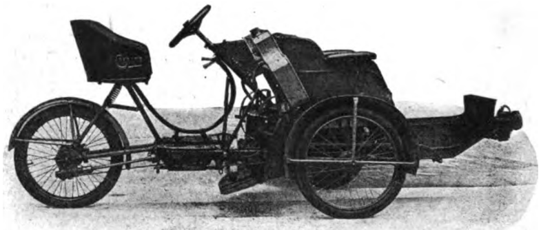
GARRARD 8-H.P. "TRI-CAR," A TYPE OF VEHICLE POPULAR IN ENGLAND.
